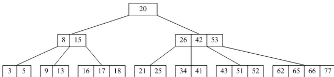
FIGURE 1 – B-tree
